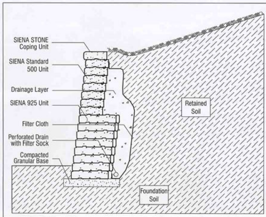
Typical Cross Section - for detailed engineering information contact Unilock®.
