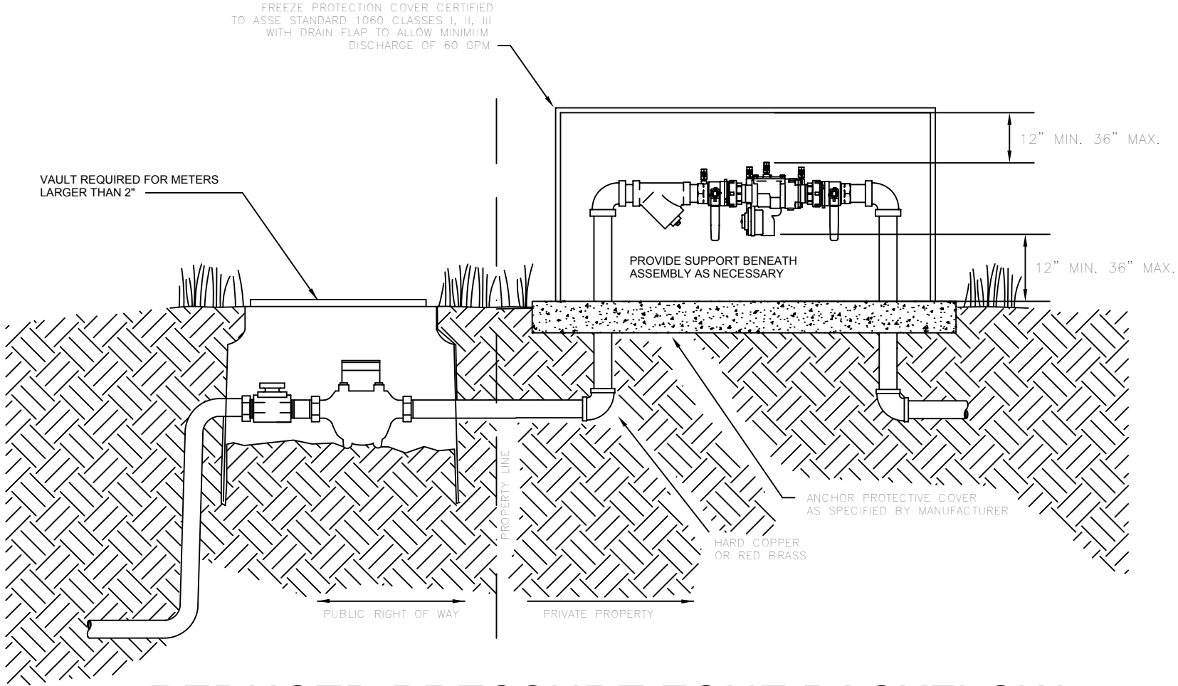
REDUCED PRESSURE ZONE BACKFLOW ASSEMBLY, OUTDOOR INSTALLATION
