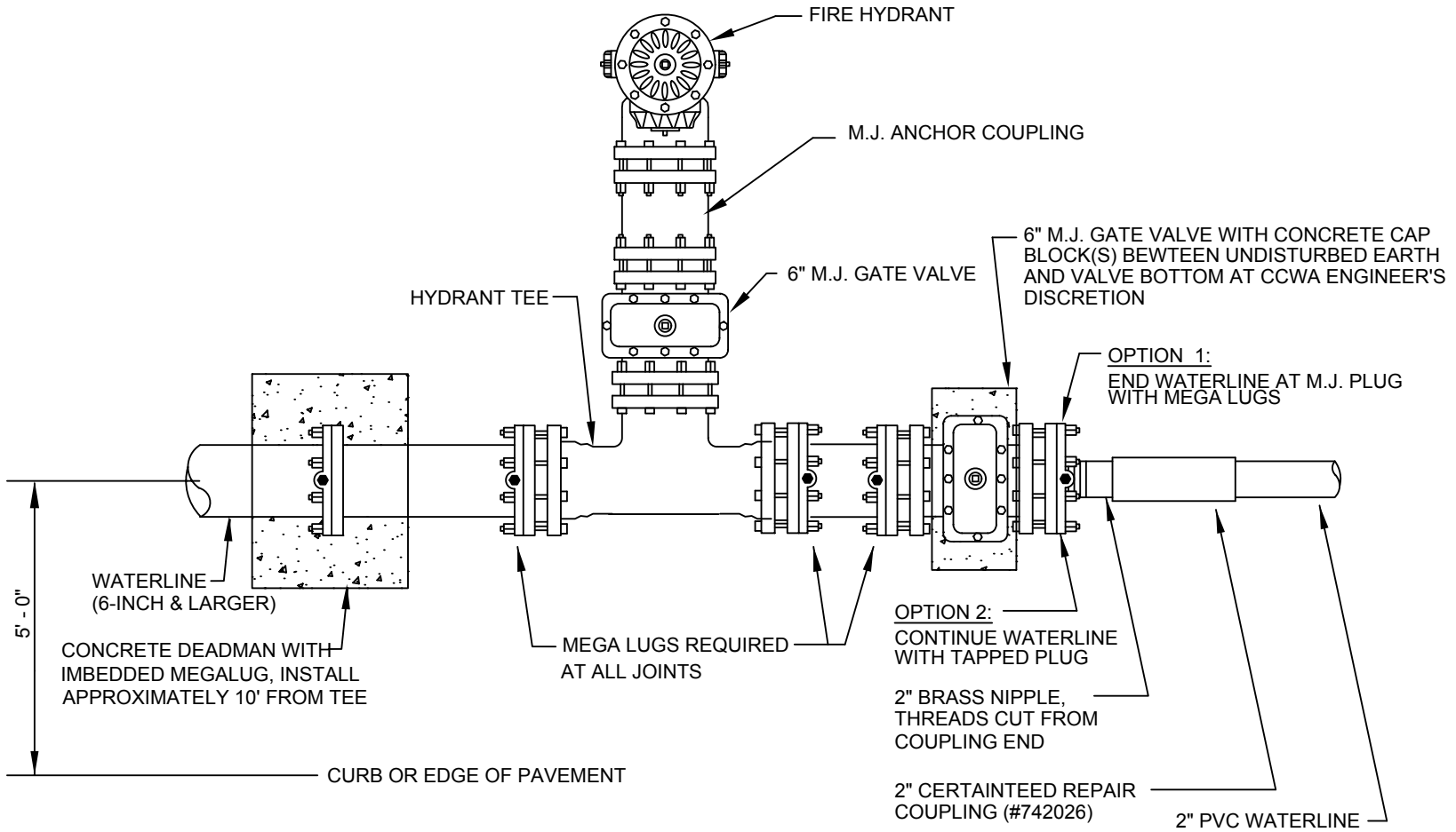
END OF LINE DETAIL, 6" AND LARGER WATERLINES
