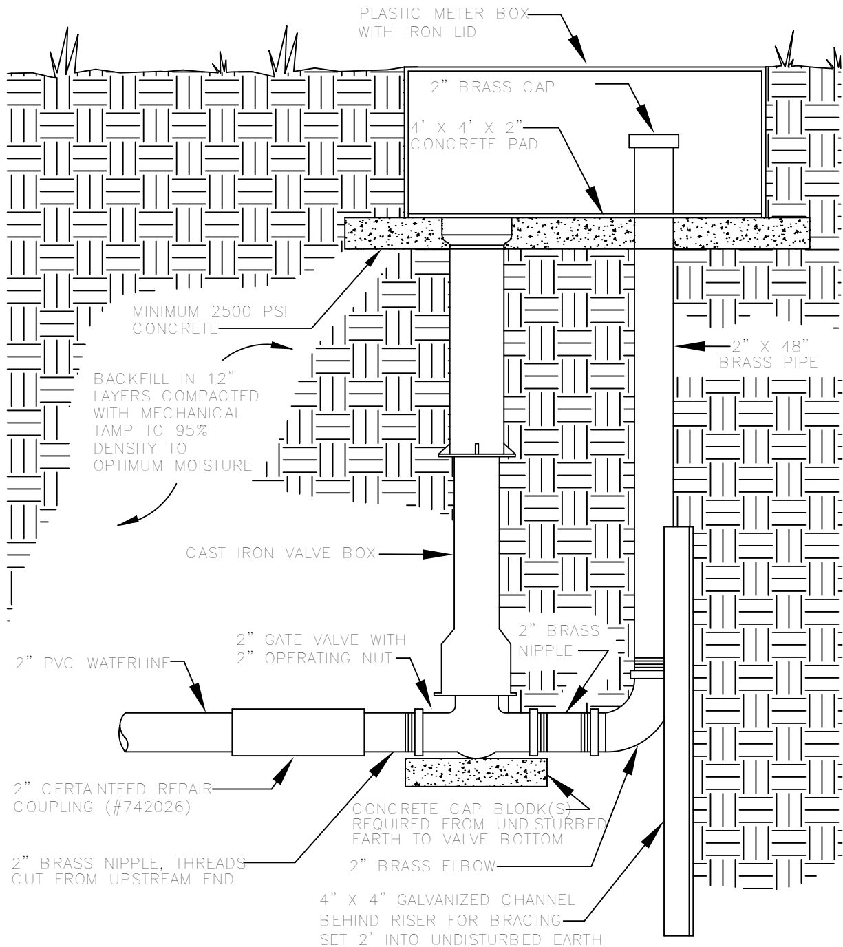
END OF LINE DETAIL, 2" PVC WATERLINES
