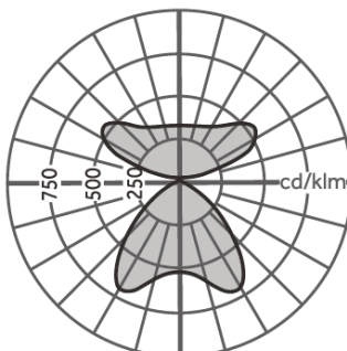
70° Direct Optic + 140° Indirect Optic
