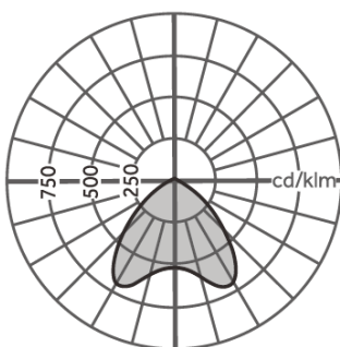
70° Direct Optic
