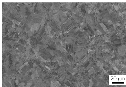
As-printed XY-plane microstructure after processing with 30 μm layer thickness and 2D energy density of 2.5 Jmm -2
