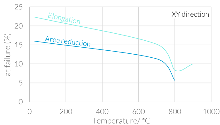
Tensile properties of ABD®-900AM after sub-solvus heat treatment. Measured in accordance to ASTM E8/E8M-16a/E21.
