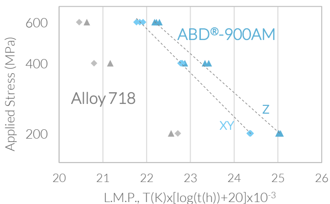
Stress rupture properties of ABD®-900AM after sub-solvus heat treatment. Measured in accordance to ASTM E139
