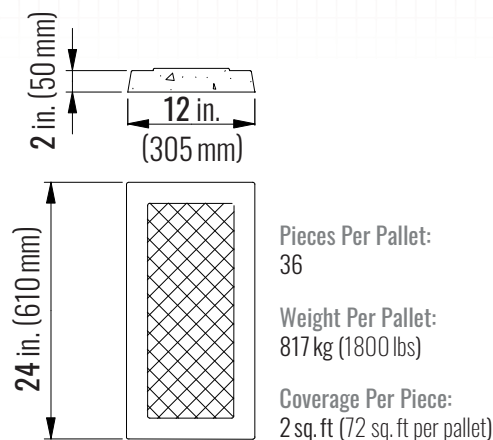
TOP VIEW / FRONT X-SECTION
