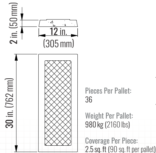
TOP VIEW / FRONT X-SECTION
