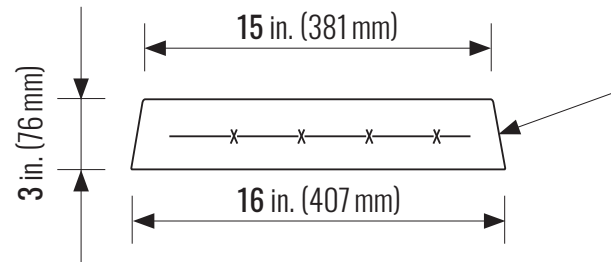
FRONT X-SECTION
