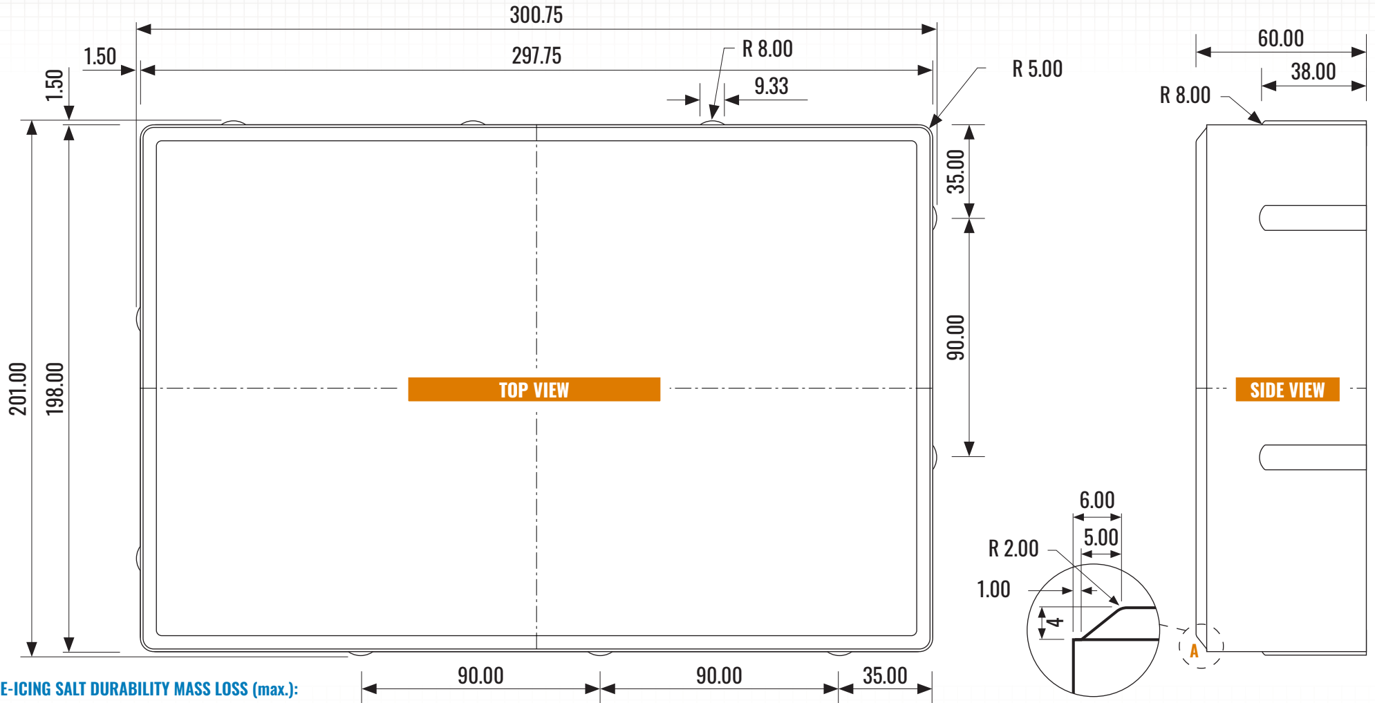
DETAIL "A" SCALE 2.9:1 ROTATED 90°
