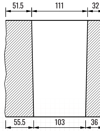
END X-SECTION
