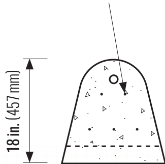
END X-SECTION
