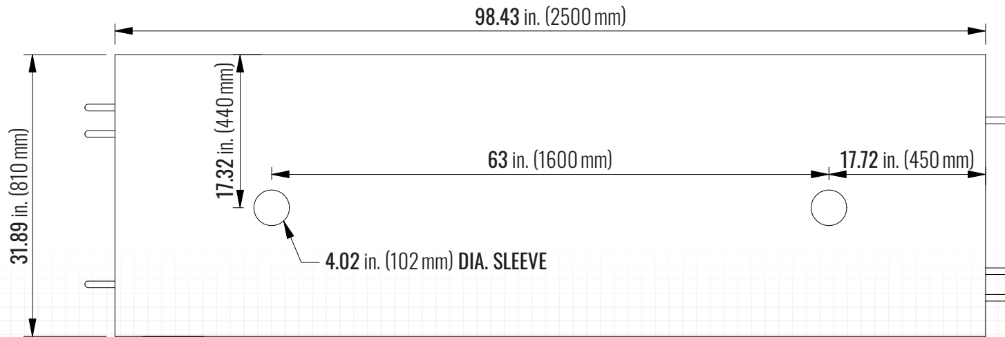
SIDE VIEW
