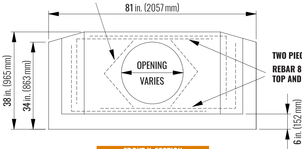
FRONT X-SECTION
