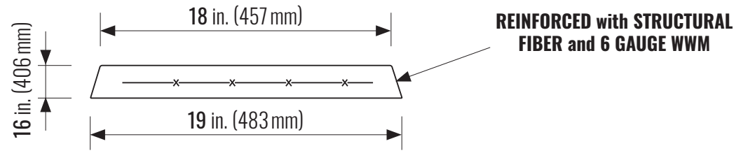
FRONT X-SECTION
