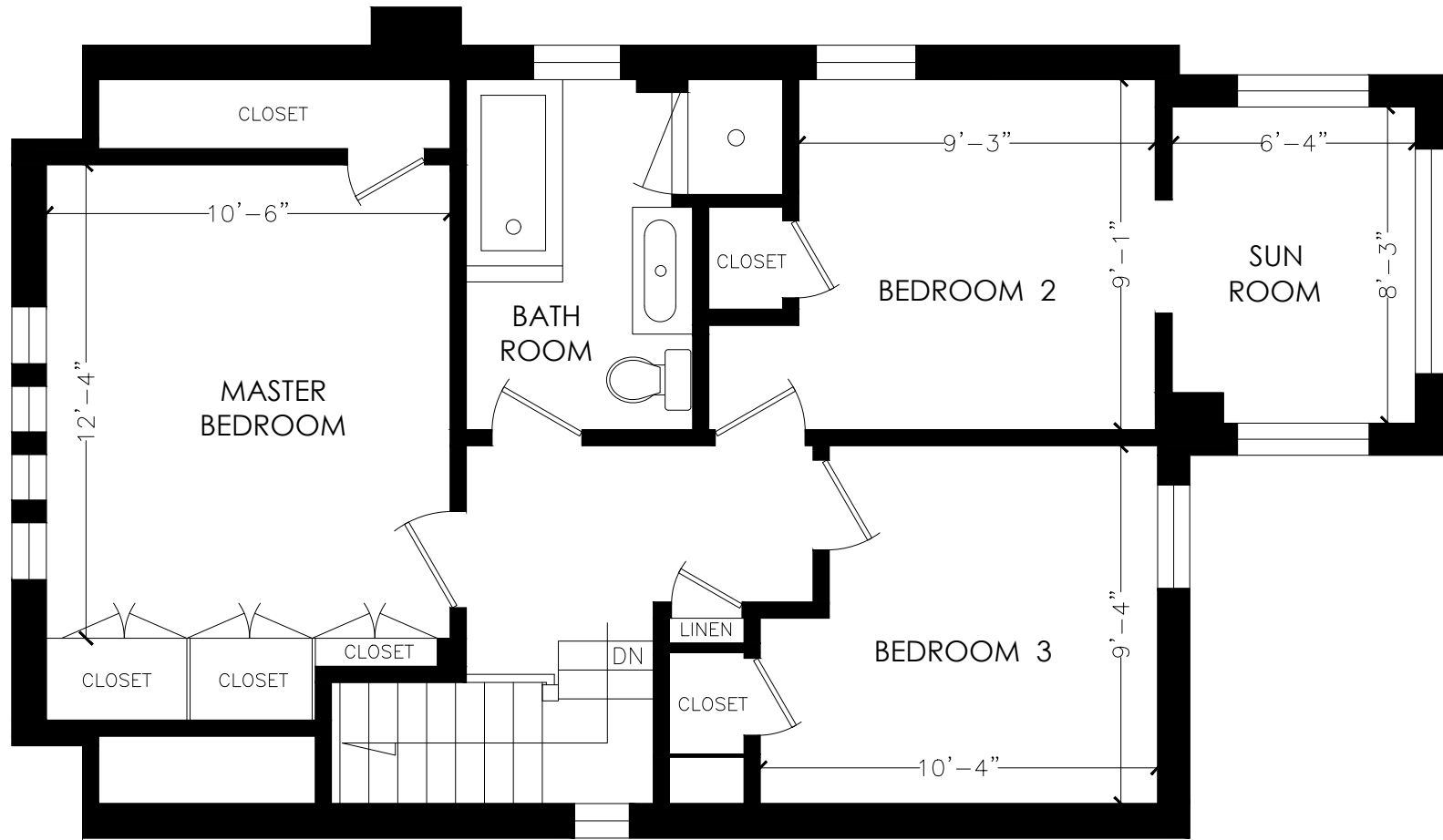
SECOND FLOOR FLOOR AREA 686 SQUARE FEET
