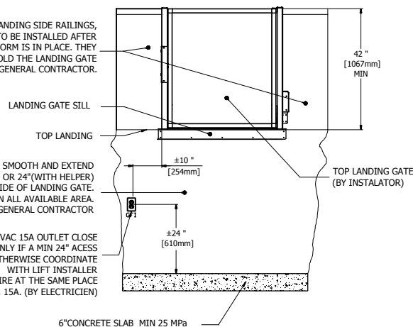
2 DETAIL A SIDE VIEW
