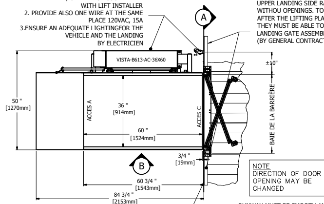
1 VISTA-613-AC 36x60 (WITHOUT HELPER)
