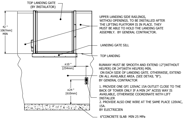
2 DETAIL A SIDE VIEW
