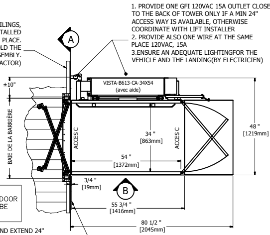
1 VISTA-613-AC 34x54 (WITH HELPER)
