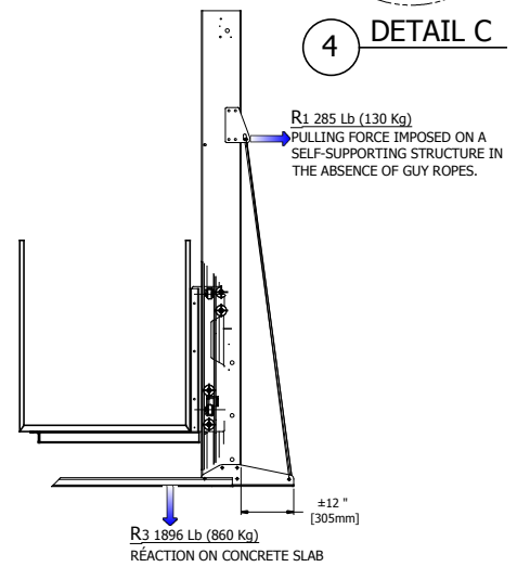
6 VISTA 1000 Lb REACTIONS
