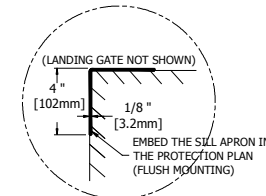
4 DETAIL C
