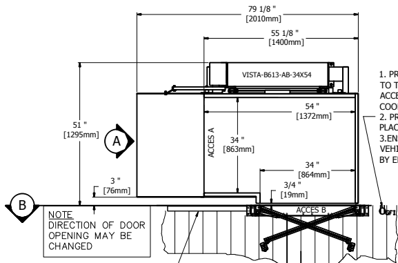
1 VISTA-613-AB 34x54 (WITHOUT HELPER)
