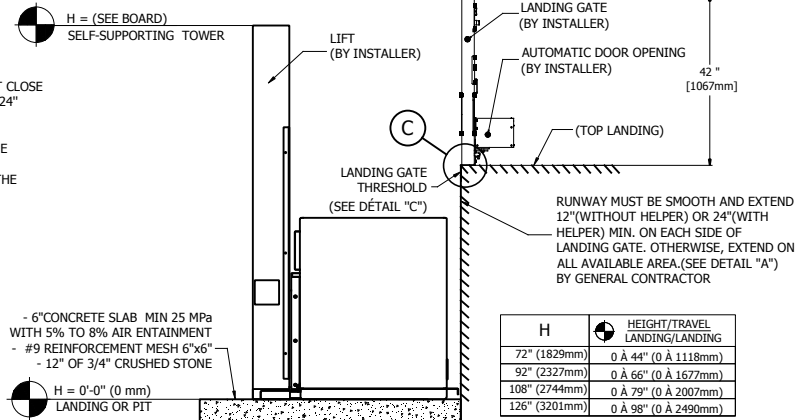
3 DETAIL A FLOOR ELEVATION
