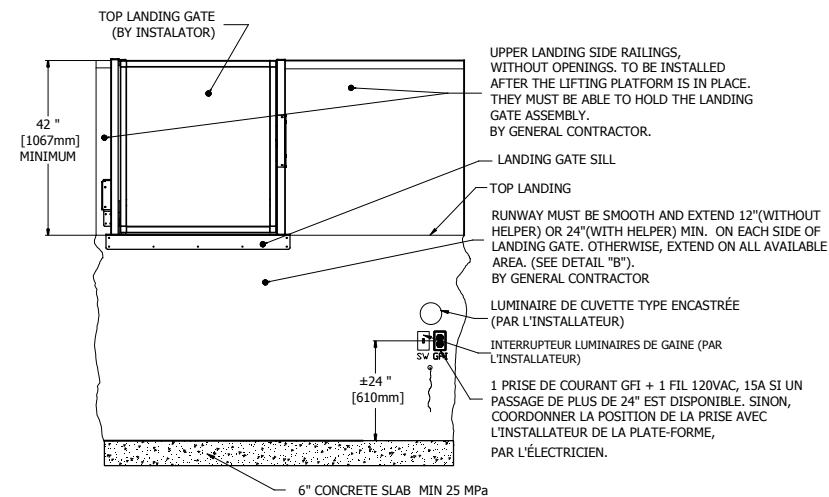
2 DETAIL B
