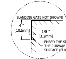
4 DETAIL C
