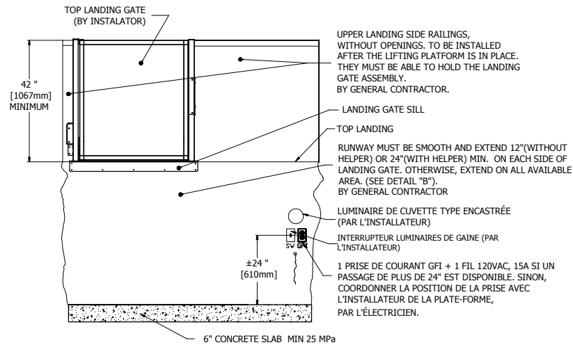
2 DETAIL B
