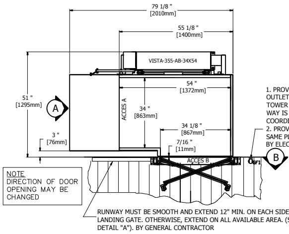
1 VISTA-355-AB 34x54 (WITHOUT HELPER)
