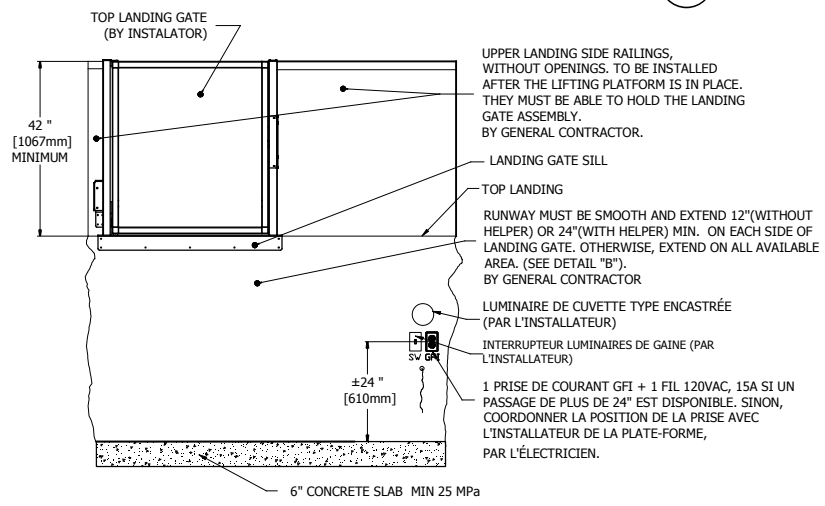
2 DETAIL B
