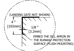
4 DETAIL C
