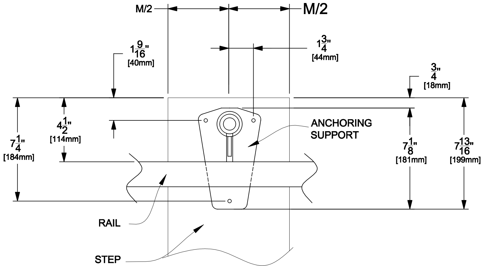
1 ANCHORING SUPPORT
