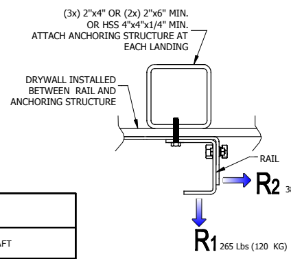
2 RAILS REACTIONS
