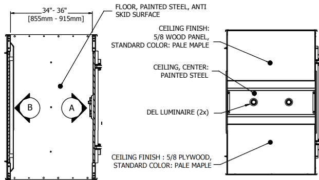
CEILING VIEW
