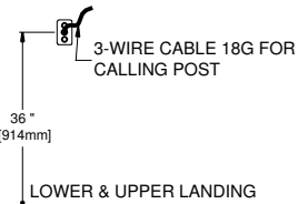
C ELECTRICAL DETAIL
