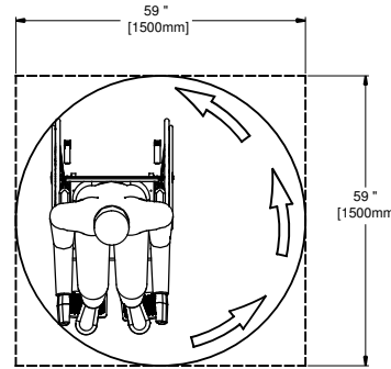
D DETAIL TURNING CLEARANCE
