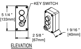
F CALL STATION SURFACE MOUNT
