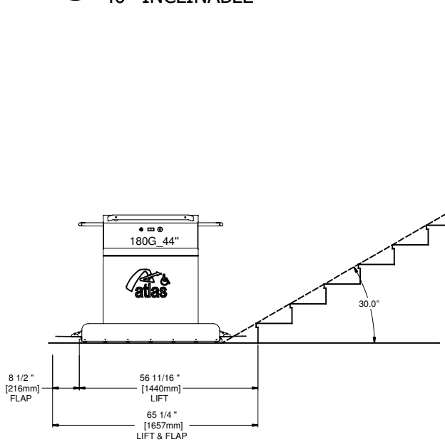
3 CLEARANCE DIMENSION 30° INCLINABLE
