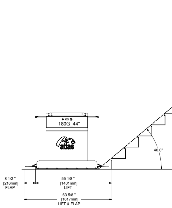
1 CLEARANCE DIMENSION 40° INCLINABLE
