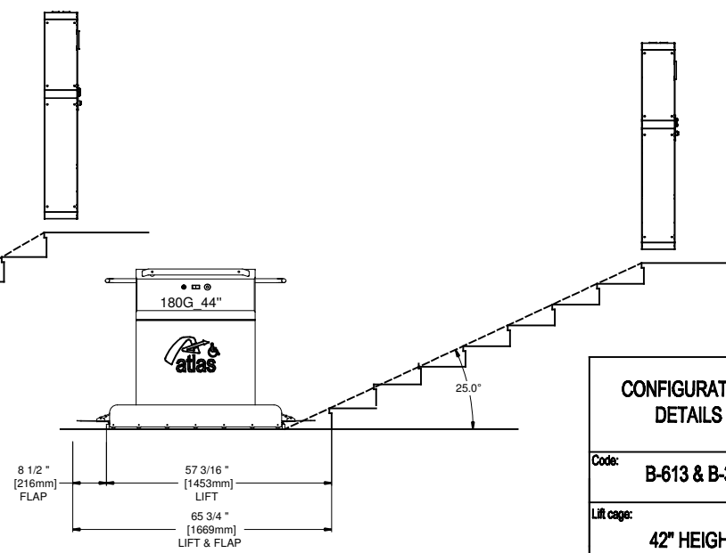
4 CLEARANCE DIMENSION 25° INCLINABLE
