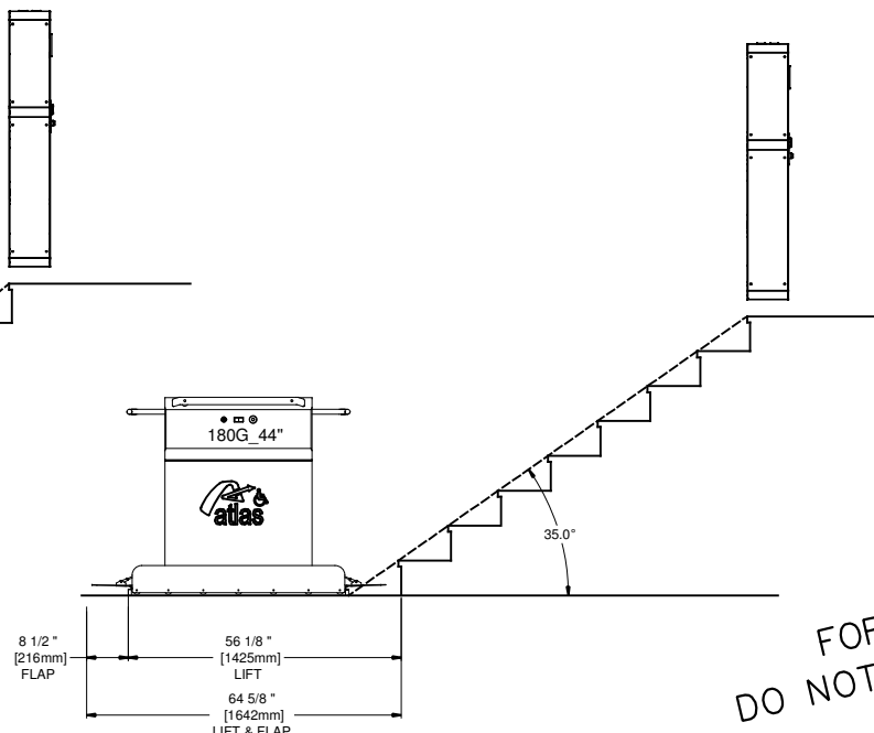
2 CLEARANCE DIMENSION 35° INCLINABLE
