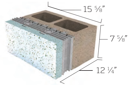
InsulTech™ Pre-Assembled Unit
