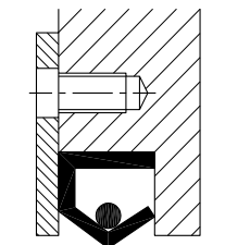
Rotary Shaft Seal
