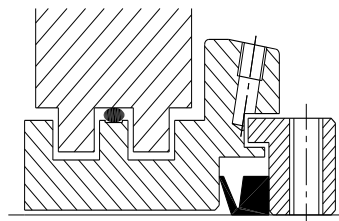
Taconite Seal A
