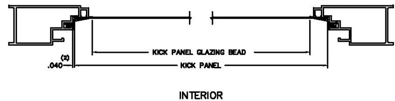
HORIZONTAL VIEW
