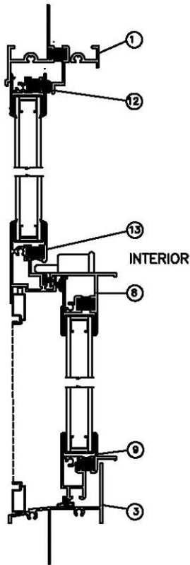
4440W THERMAL BREAK
