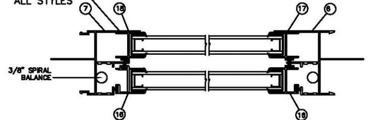
4400W REMOVABLE FIXED LITE
