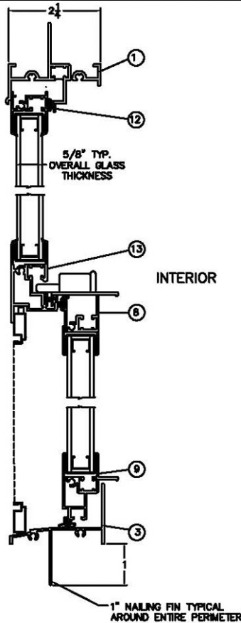
4400W REMOVABLE FIXED LITE
