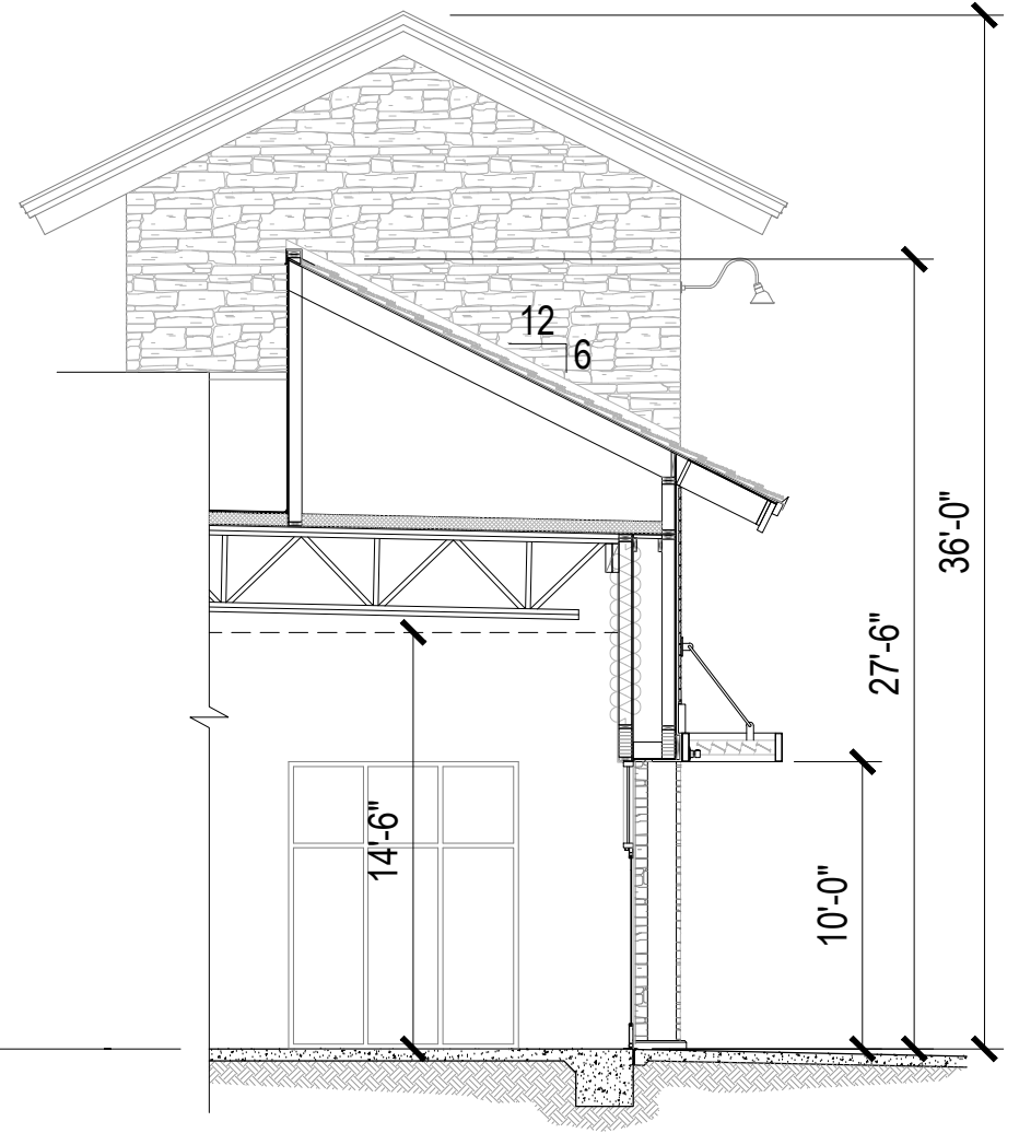
SECTION 2
