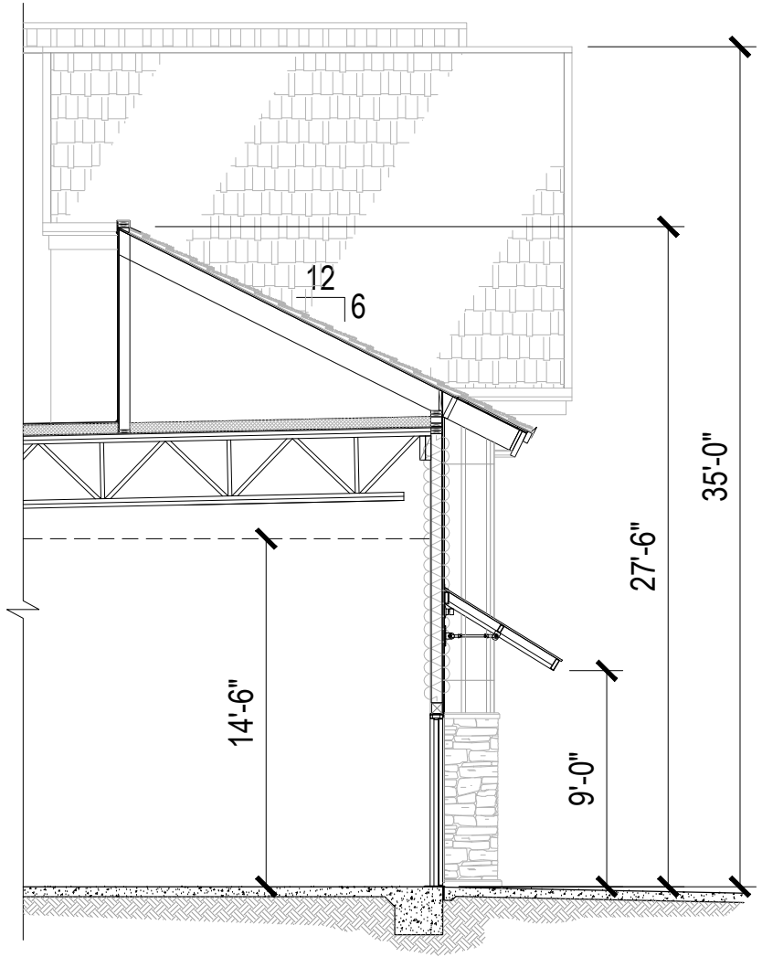
SECTION 1
