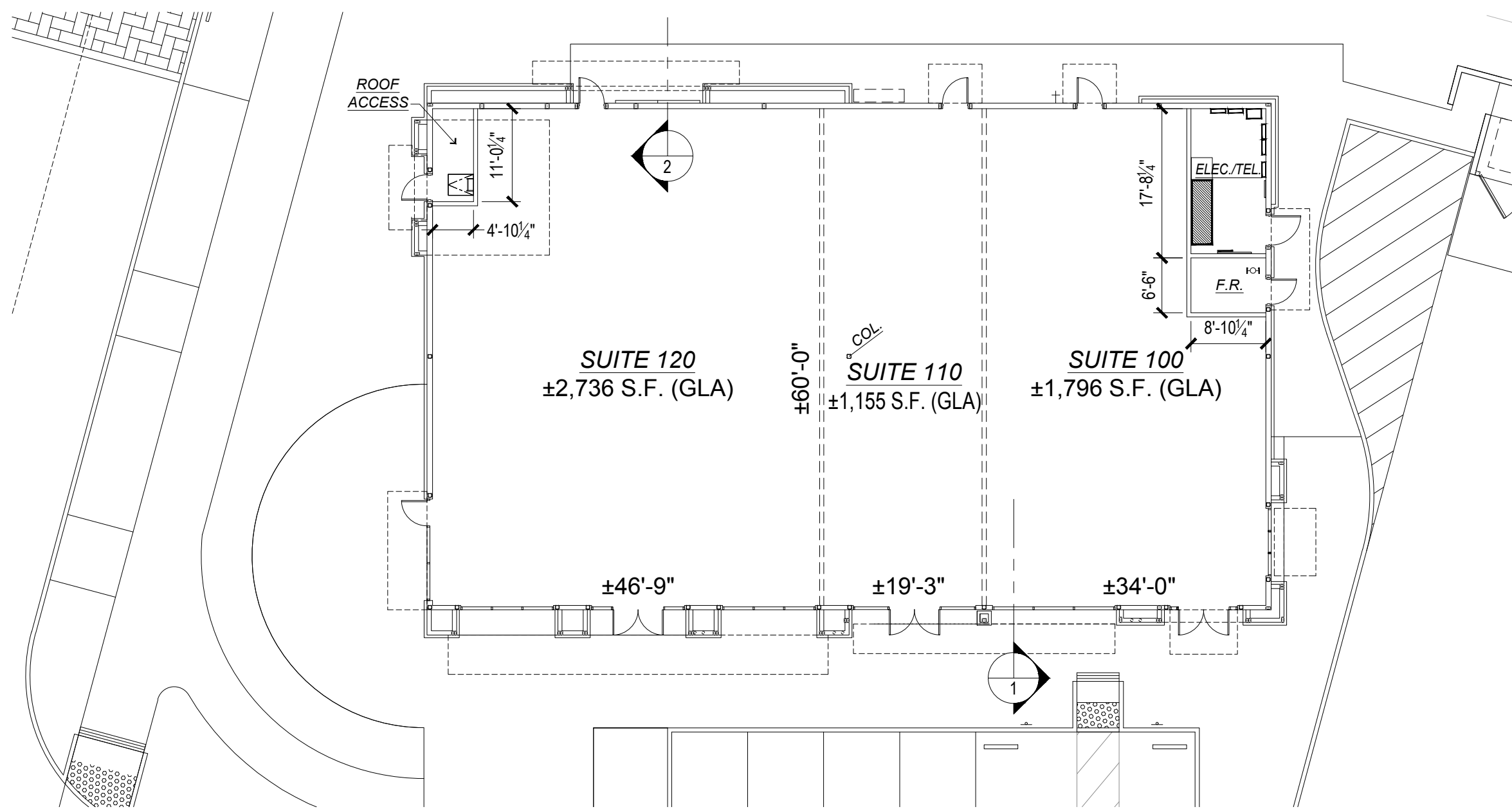
FLOOR PLAN
