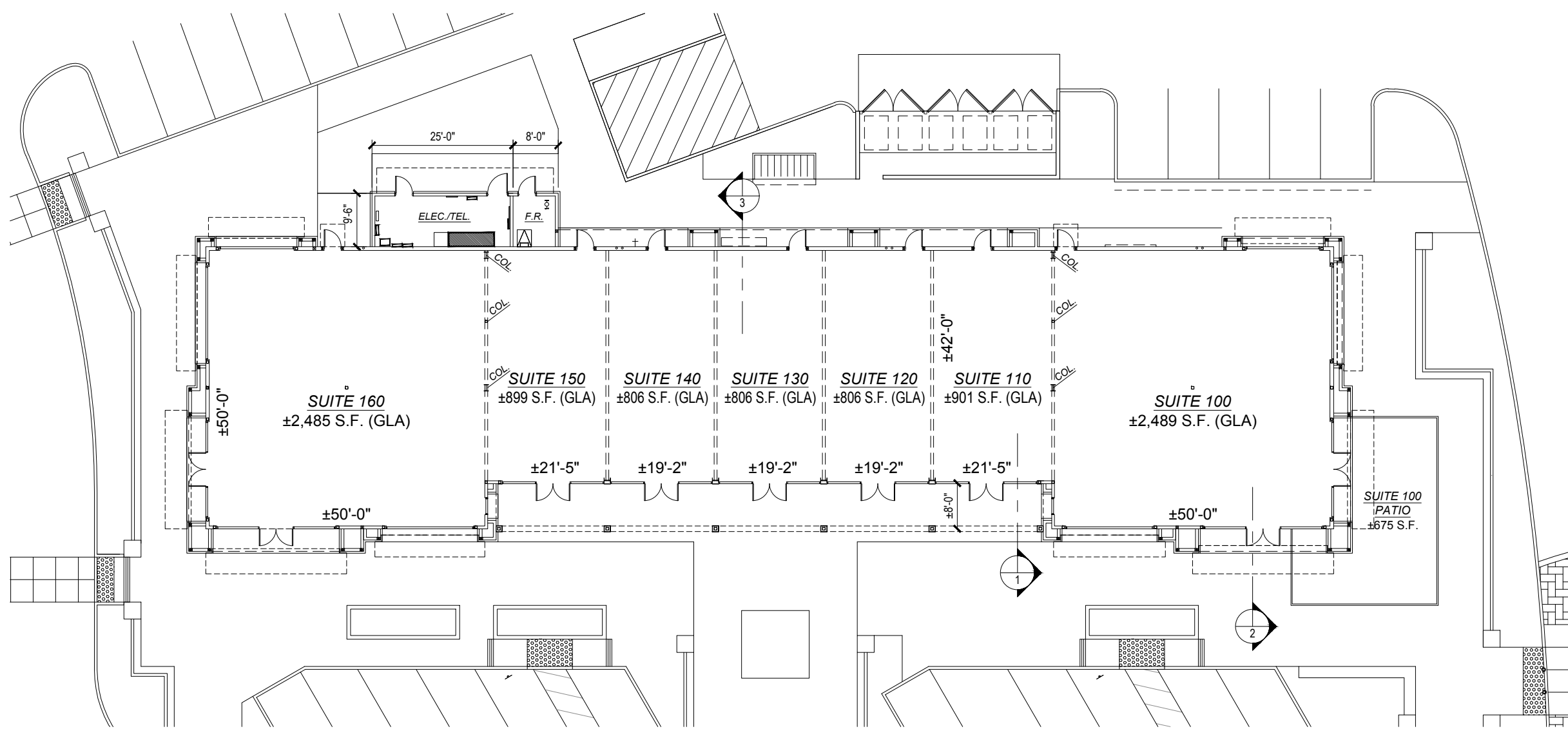
FLOOR PLAN
