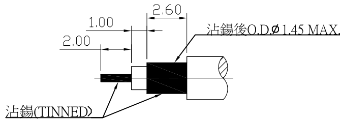
RECOMMENDED CABLE STRIPPING DIM'S (建議剝線尺寸)
