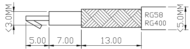
RECOMMENDED CABLE STRIPPING DIM'S (建議剝線尺寸)
