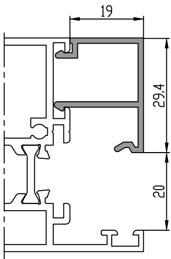
51 5040 10: 0.236 kg/m 51 5040 14: 0.323 kg/m
