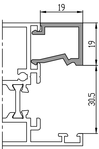
51 5041 18: 0.325 kg/m
