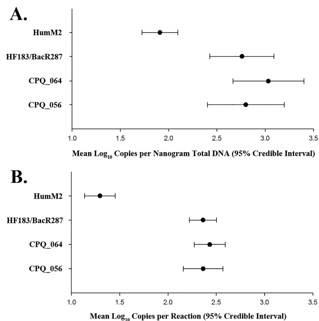
Figure 2. Abundance of crAssphage and bacterial human-associated qPCR targets in primary influent sewage (panel A) and environmental water samples (panel B). Values are reported as mean \log_{10} copies estimates per nanogram of total DNA (panel A) or per reaction (panel B) with 95% credible intervals. Sewage qPCR reactions contained 1 ng of template DNA extracted from 10 mL of wastewater, while environmental water qPCR reactions contained 2 \mu L of DNA extracted from a total volume of 200 mL of impacted water.
