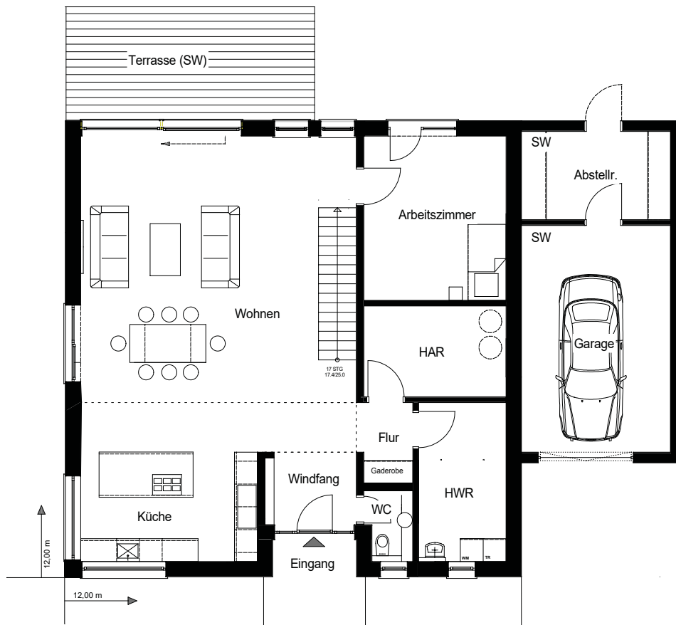
T04-01-Erdgeschoss
