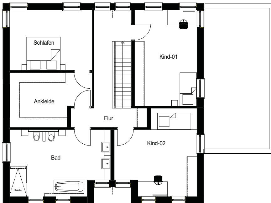
T04-02-Obergeschoss
