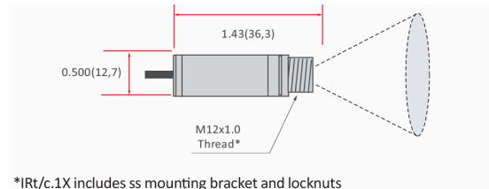
*IRt/c.1X includes ss mounting bracket and locknuts Dimensions are in inches (mm)
