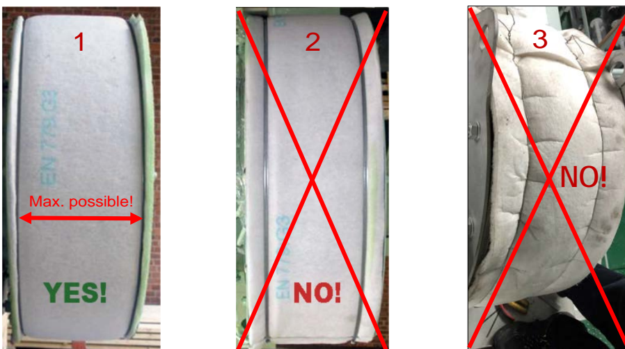
Figure 4: Correct (1) and not correct assembled MAN OEM air filter mat (2), (3).
