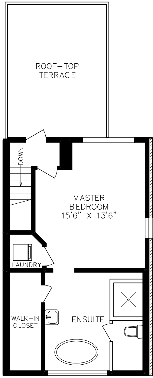
THIRD FLOOR 524 SQUARE FEET
